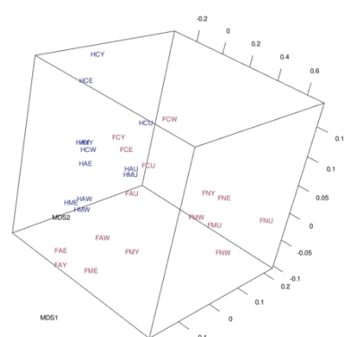
Fig: MDS analysis, projected in 3 dimensions.
